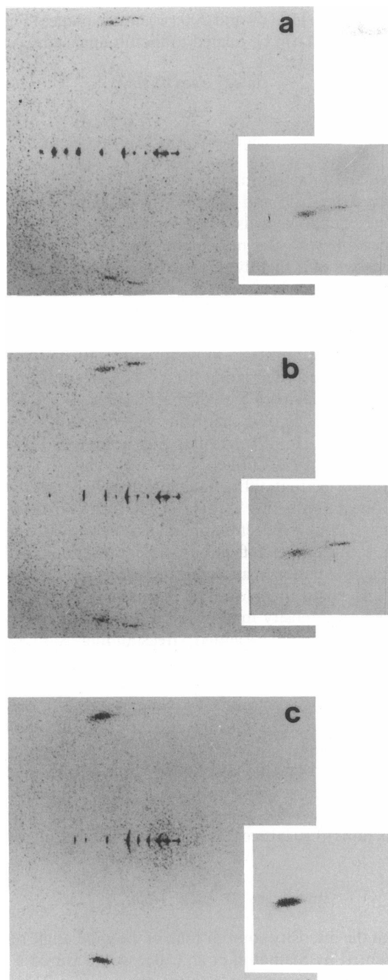
FIGURE 1 X-ray diffraction patterns at 25°C of oriented DPPC multilayers at (a) 0% RH having a d -spacing of 55.2 Å and \phi and \psi angles of 21.5° and 11.4°, respectively, corresponding to a chain tilt angle \theta of 21.5°. (b) 70% RH bilayers ( d -spacing of 57.9 Å) with \phi and \psi angles of 25.5° and 13.1°, respectively, implying a \theta of 25.5°. (c) 100% RH sample with a d -spacing of 58.9 Å and a \theta of 29.0° ( \phi = 26.3^\circ ).
