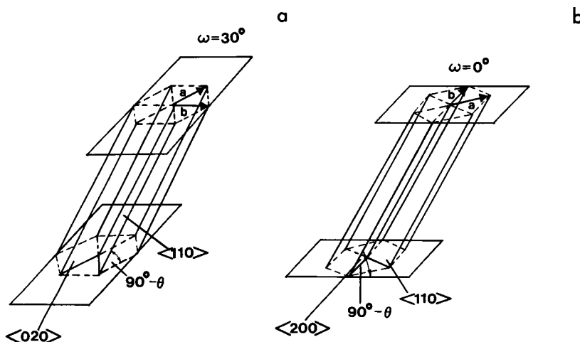
FIGURE 3 Three-dimensional representation of hexagonally packed hydrocarbon chains tilted (a) along one of the basic hexagonal lattice vectors ( \omega = 30^\circ ), or (b) along one of the bisectors ( \omega = 0^\circ ) of the hexagonal lattice. From the schematic, one can observe that the 200 and 110 planes are tilted with respect to the planes of the bilayer while the 020 is perpendicular.
