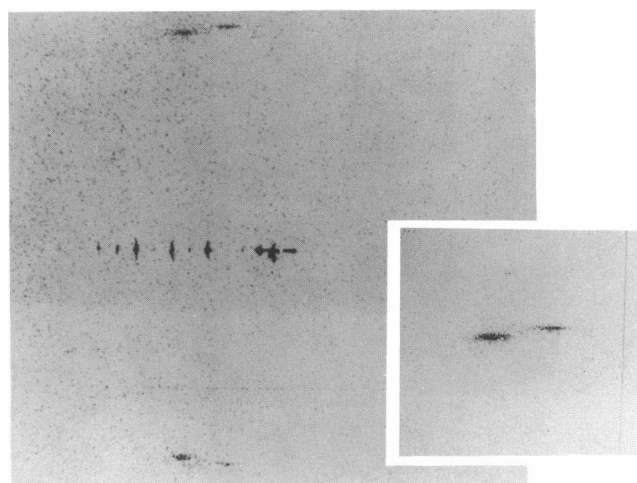
FIGURE 4 X-ray diffraction pattern of oriented DPPC multilayers annealed for 1 wk at room temperature and ≈40% RH after exposure to the liquid-crystalline phase. The measured \phi and \psi angles are 21.8° and 11.4°, respectively, with the bilayers having a d -spacing of 57.5 Å.
